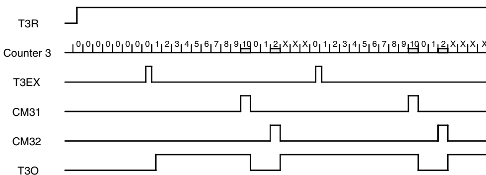
Figure 49. Externally Triggered Counter Reset and Start Combined with Single-action Mode
