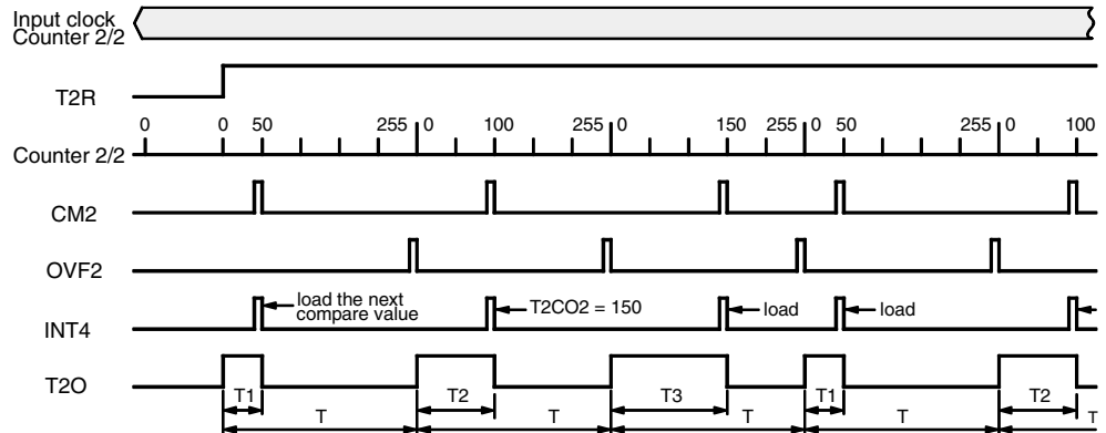
Figure 42. PWM Modulation
